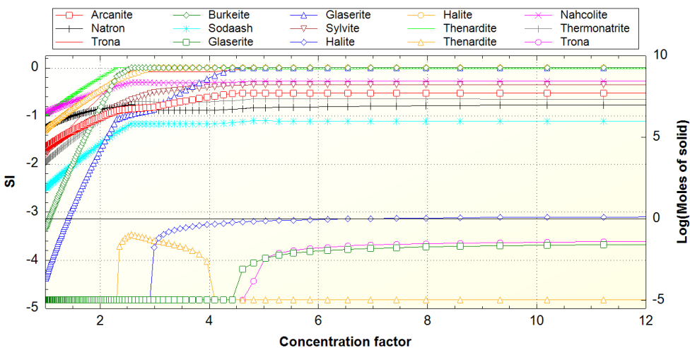
Figure 3 Saturation Indices and Moles of solid posted during evaporation at 30°C
