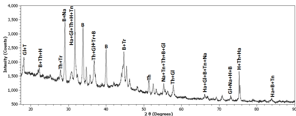
Figure 1 XRD Pattern of mineral precipitates (Gl-Glaserite, Th-Thenardite, Ha-Halite, Tr-Trona, B-Burkeite, Na-Natron, Tn-Thermonatrite, H-Hanksite).
